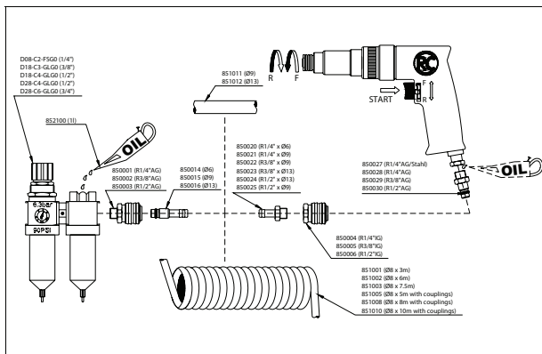
Screwdriver - Rodcraft 4700
